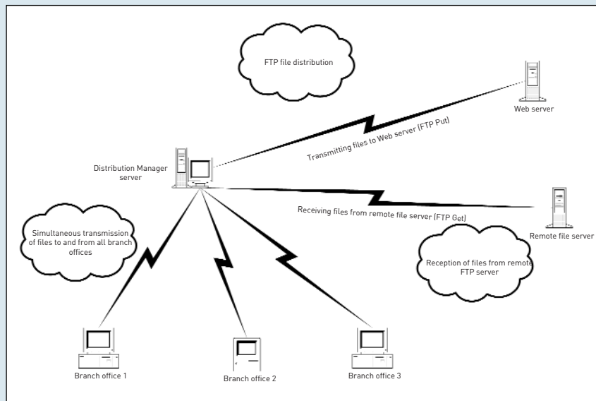
Distribution Manager flowchart.
